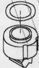
(KG7-M711E-C0X) PICK-UP NOZZLE E, COMP (TYPE 34) YAMA, YVL88 (KMO-M711E-00X)
